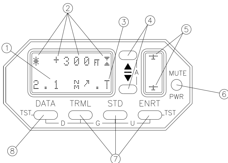
Figure 5. ½ 3ATI Traffic Display After Traffic Acquisition
